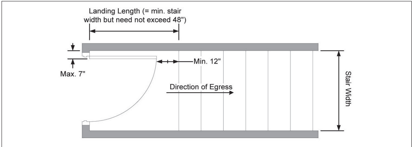
FIGURE 1008.1.5(1) (LANDING DIMENSIONS ONLY)
