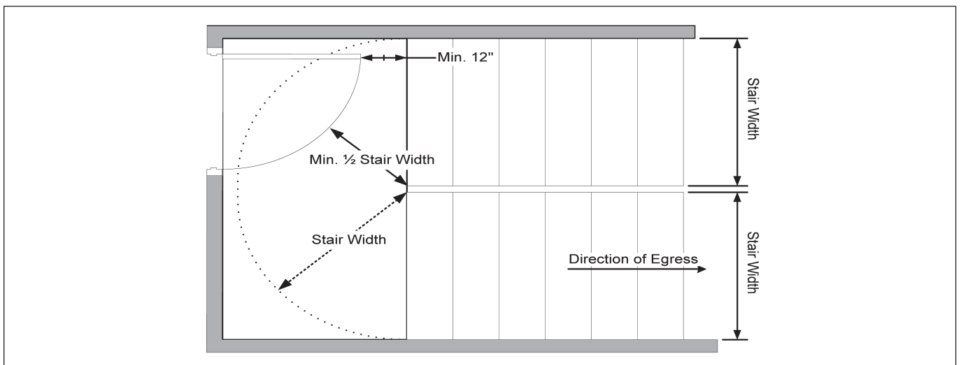
FIGURE 1008.1.5(3) (LANDING DIMENSIONS ONLY)
