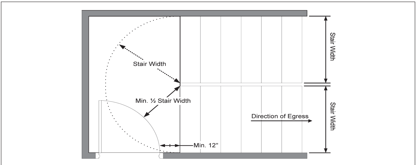
FIGURE 1008.1.5(2) (LANDING DIMENSIONS ONLY)
